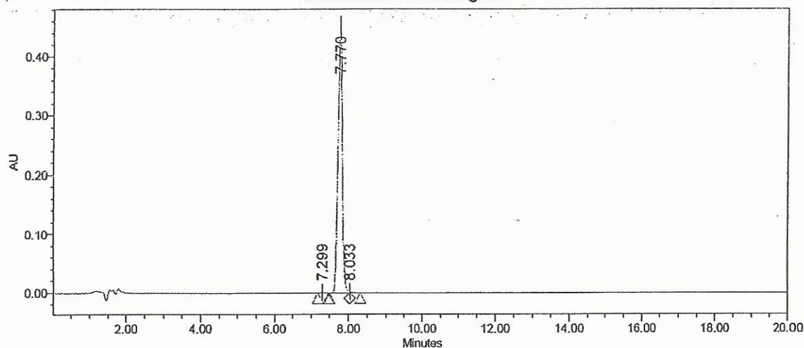
Auto-Scaled Chromatogram
